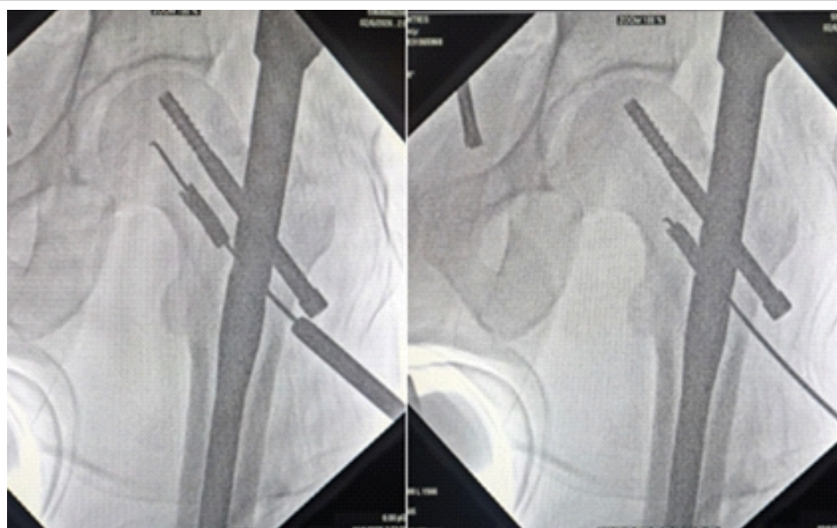
Figure 3: Performing the lever maneuver with depth gauge. Intraoperative fluoroscopic images demonstrating the depth-gauge lever maneuver used for retrieval of the broken drill-bit fragment. The hooked tip is engaged with the inner surface of the fragment, allowing controlled extraction through the proximal femoral nail.
