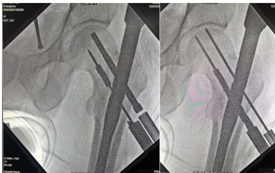
Figure 1: Fractured drill bit at mid-shaft, leaving the distal portion lodged within the reamed canal in the femoral neck. Intraoperative fluoroscopic image showing the fractured 8-mm cannulated drill bit with the distal fragment lodged within the femoral neck during proximal femoral nailing. The retained fragment lies along the compression-screw trajectory and necessitates retrieval to permit optimal implant positioning.
